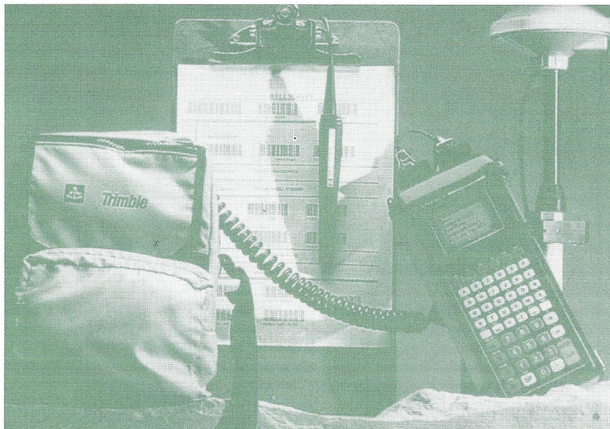
Figure 3. Typical GPS equipment needed for field surveying
