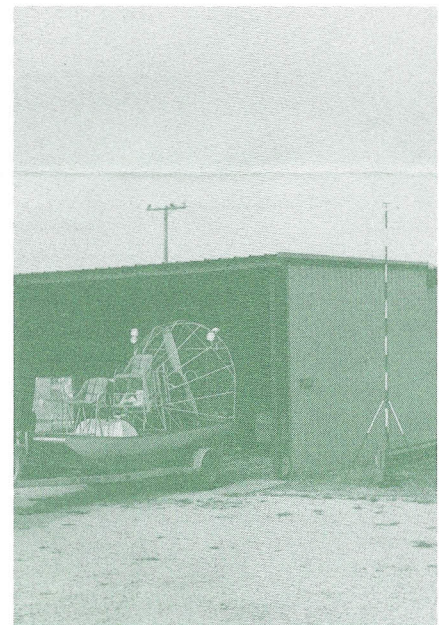
Figure 8. Base station at Lake Seminole was set up near the boat shelter. The antenna is mounted on a range pole extending above the shelter
